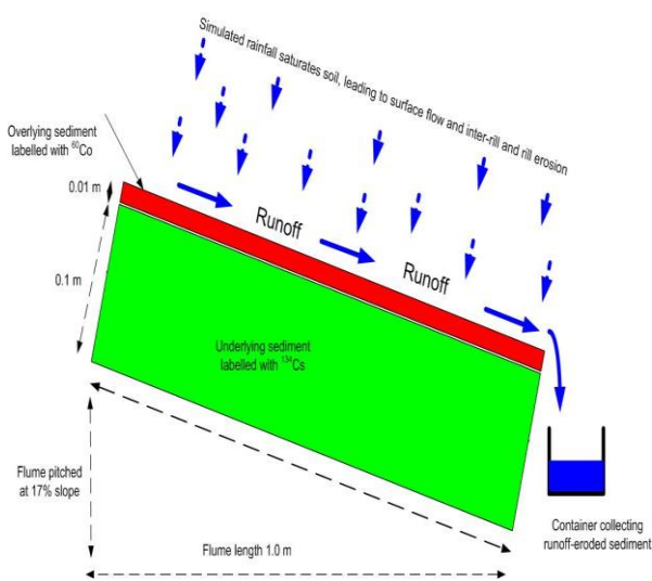
Figure 5. The stratified configuration of the two layers of labelled soil in the erosion plot.
